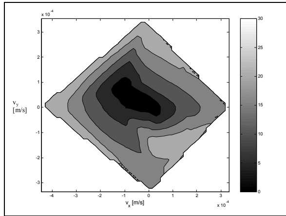
Fig. 6: Relative overall error [in %] of position controller with respect to v_x and v_y
