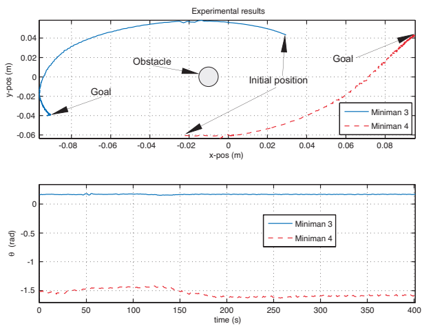
Fig. 9 Experimental results for the same initial conditions as for the simulation case
