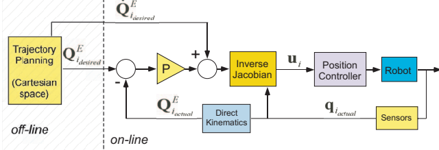
Fig. 4. Trajectory tracking control loop
