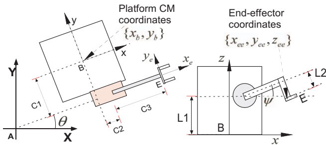
Fig. 3 Platform's top and lateral view
