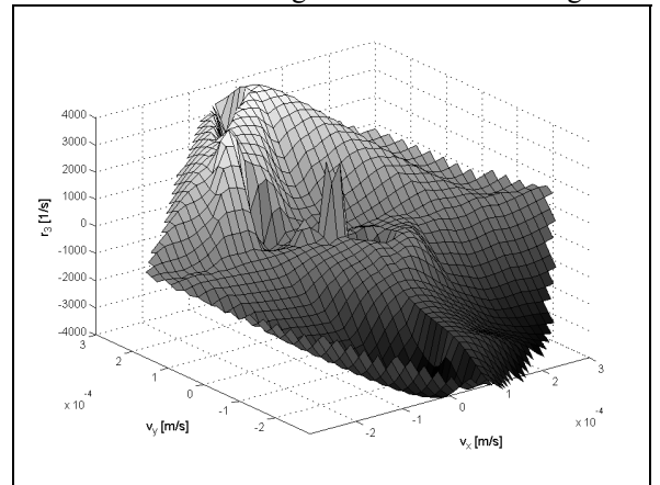
Fig.5: The frequency of one of the robots actuators with respect to v_x and v_y at constant voltage. All other actuators are deactivated (no signal)
