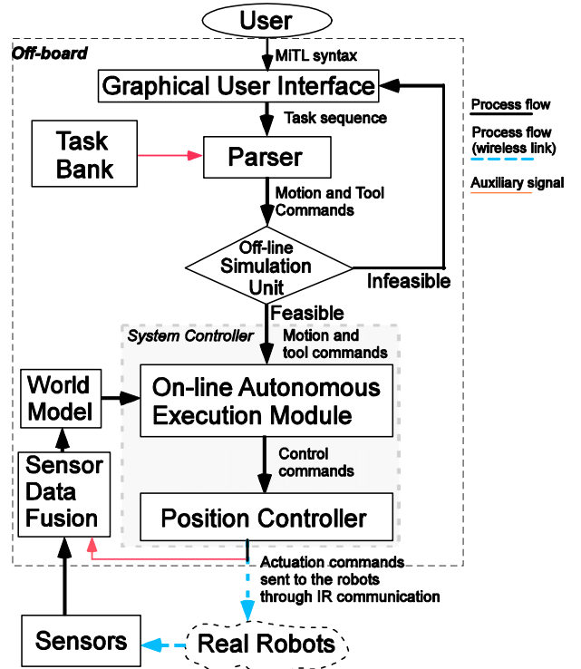
Fig. 2. MiCRoN system architecture flow diagram
